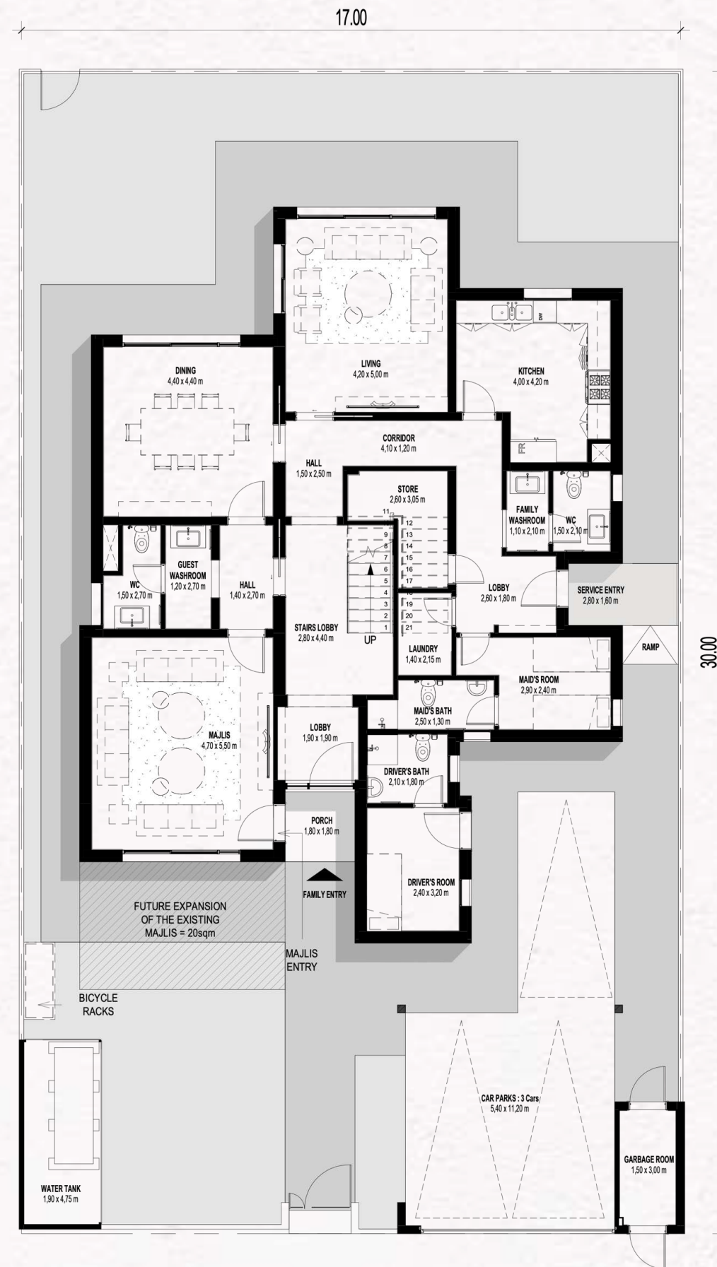
GROUND FLOOR
