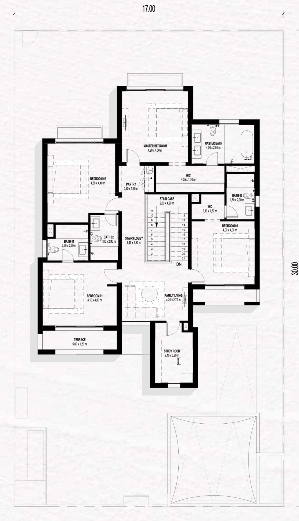
FIRST FLOOR
