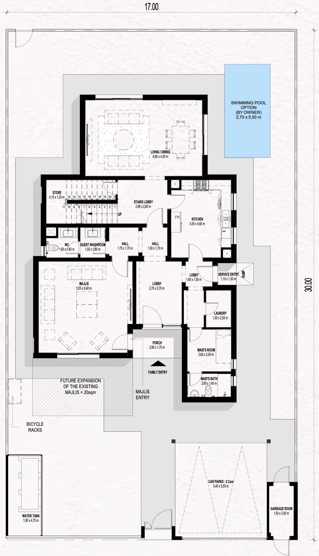
GROUND FLOOR
