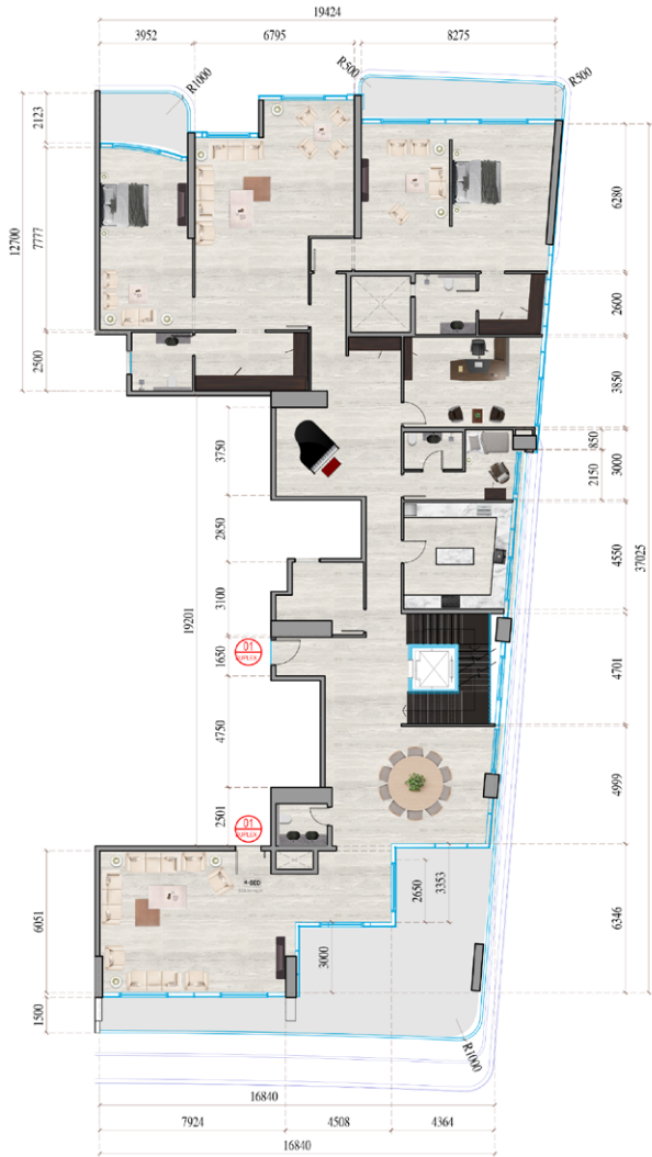
1 47th FLOOR PLAN DUPLEX 1 - LOWER FLOOR
