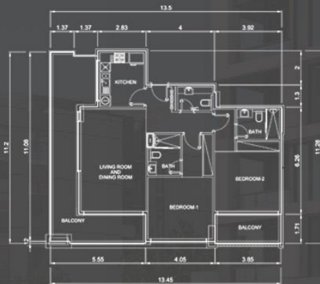
MAIN FLOOR
