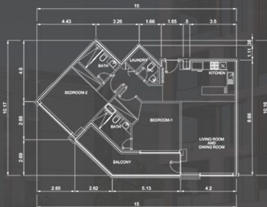
MAIN FLOOR
