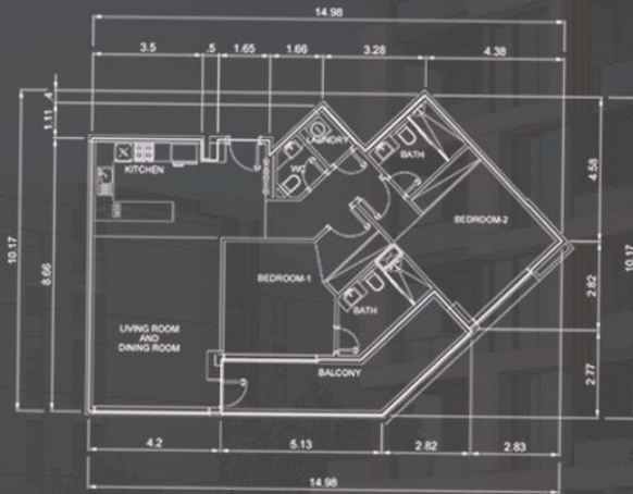
MAIN FLOOR
