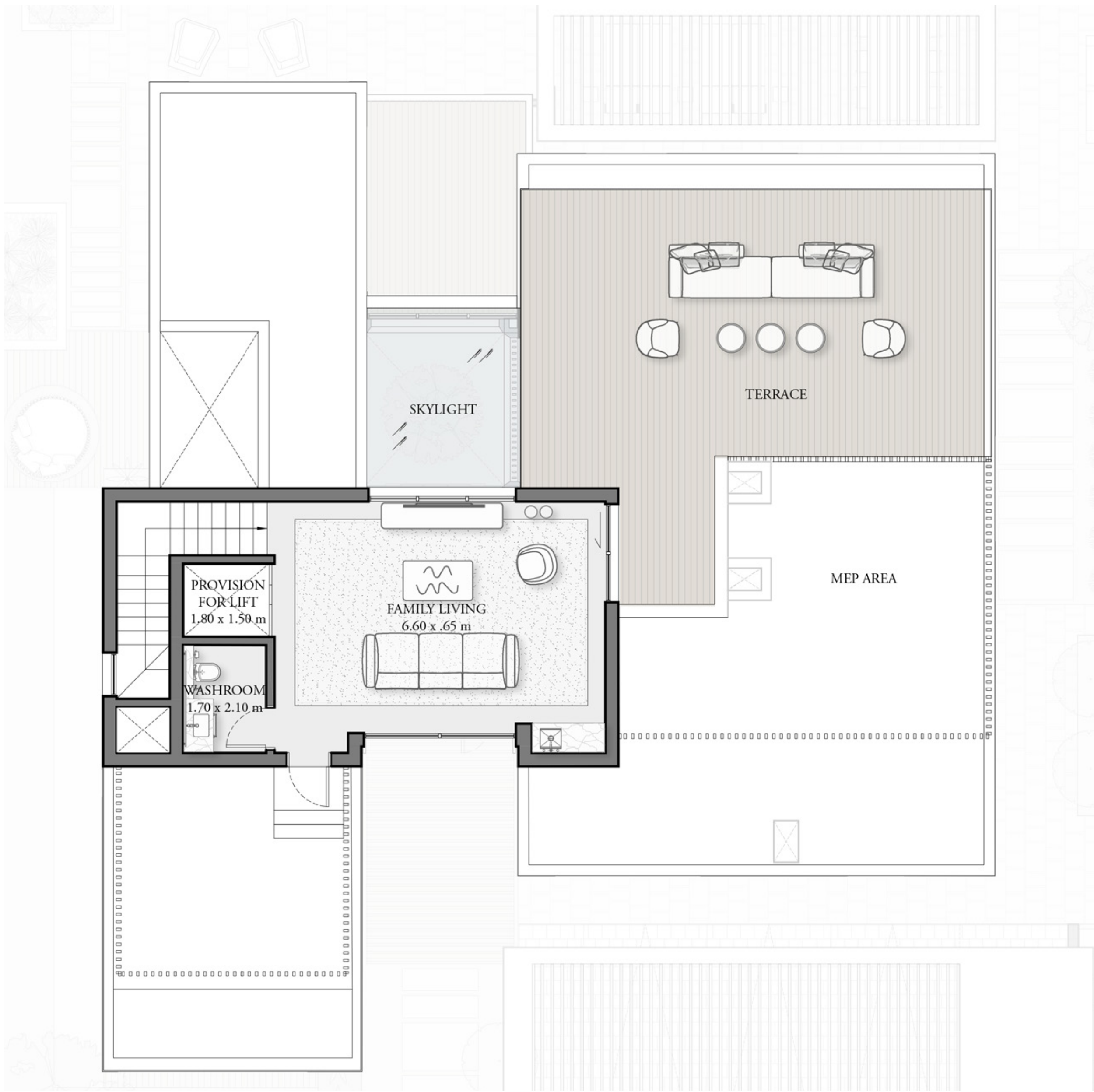
ROOF FLOOR
