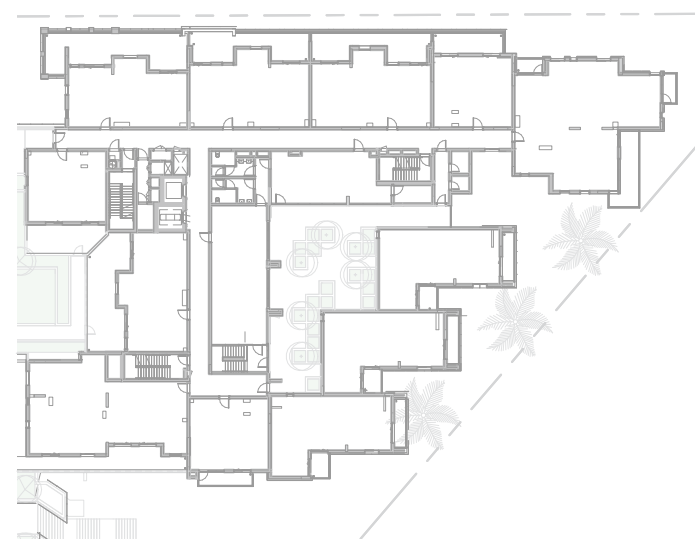
LEVEL 01
