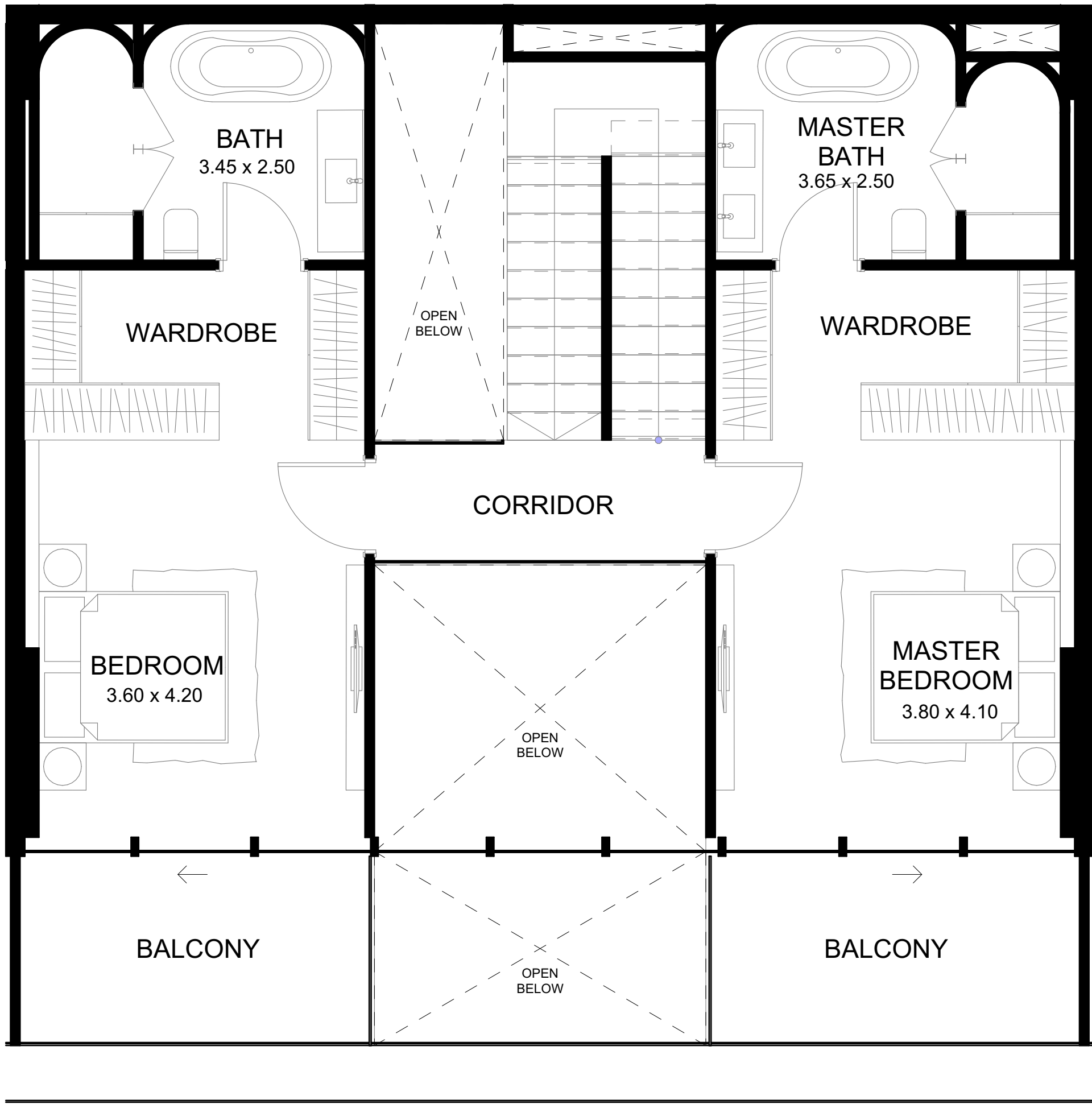
UPPER FLOOR PLAN
