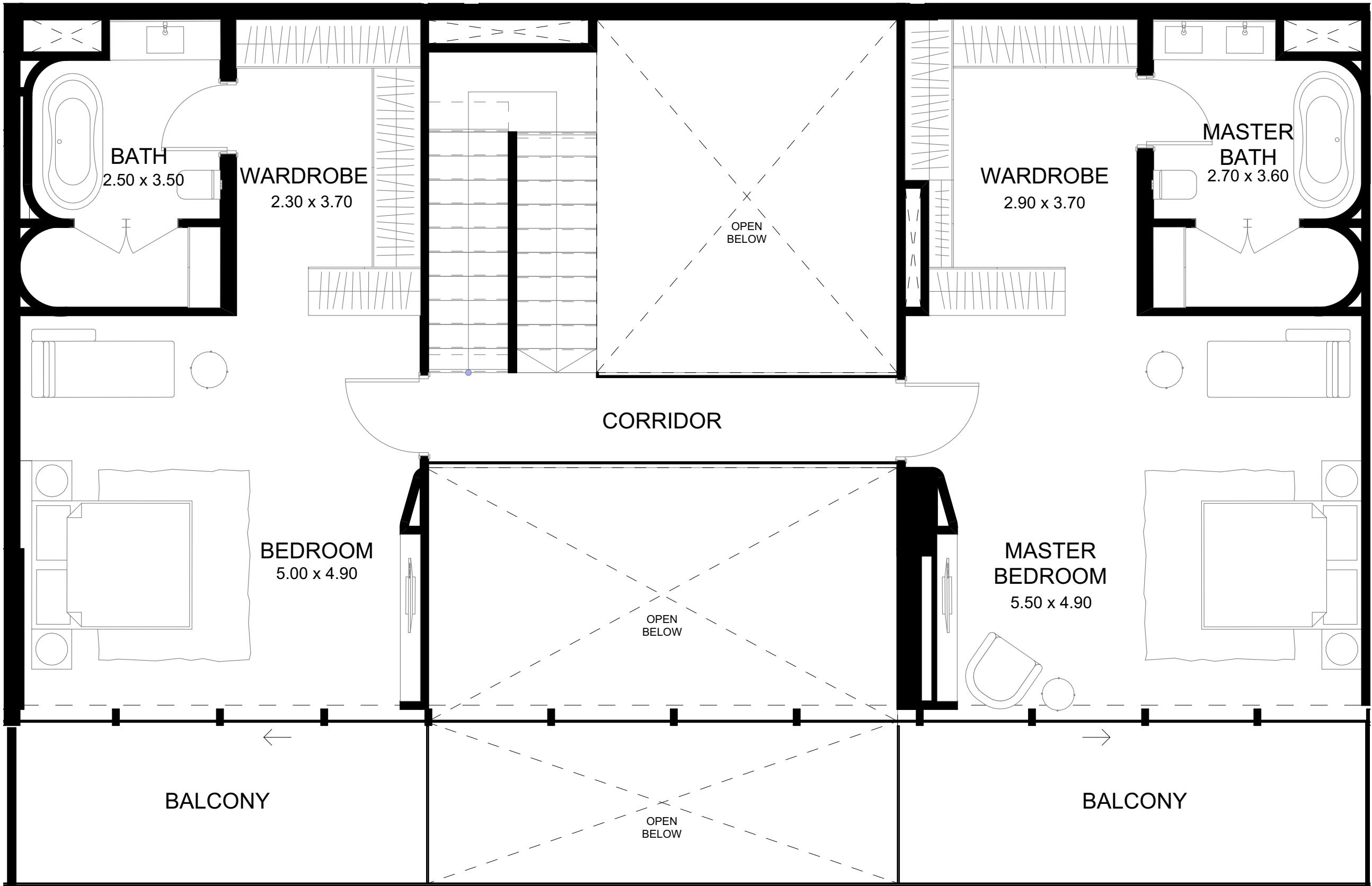
UPPER FLOOR PLAN
