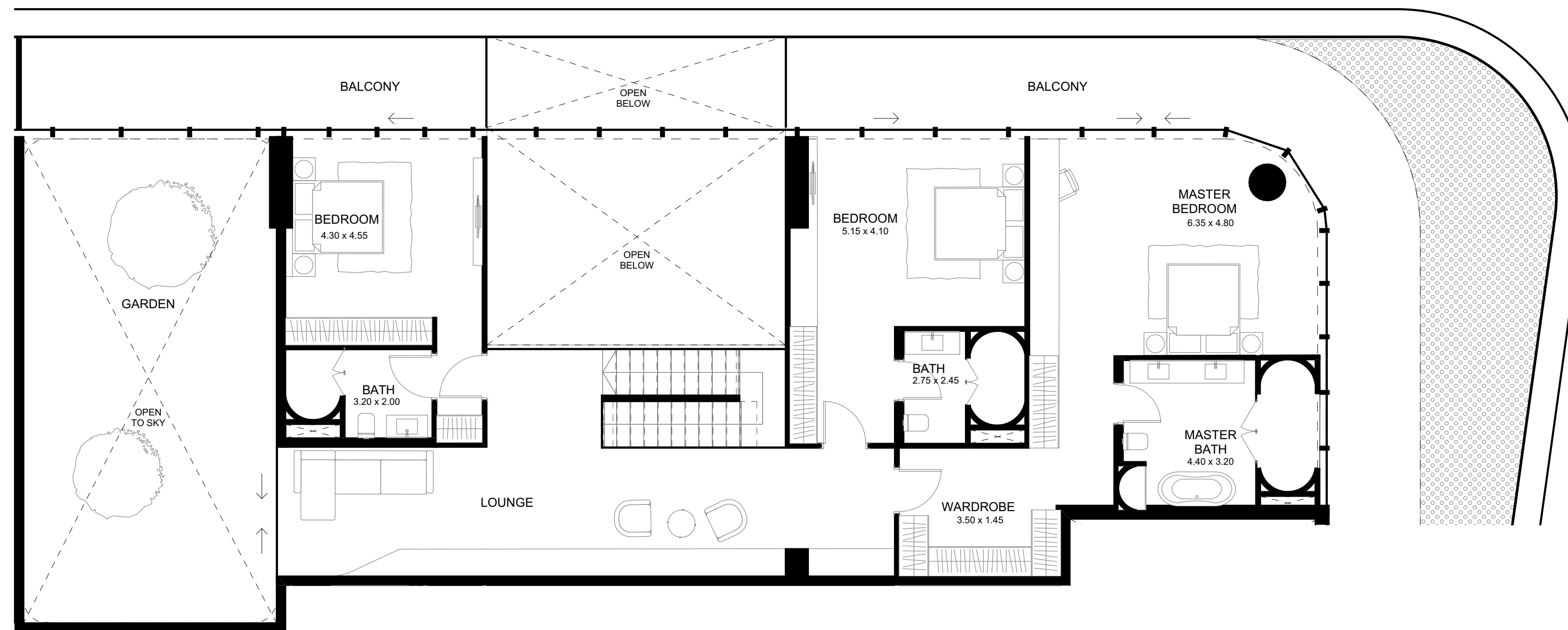
UPPER FLOOR PLAN
