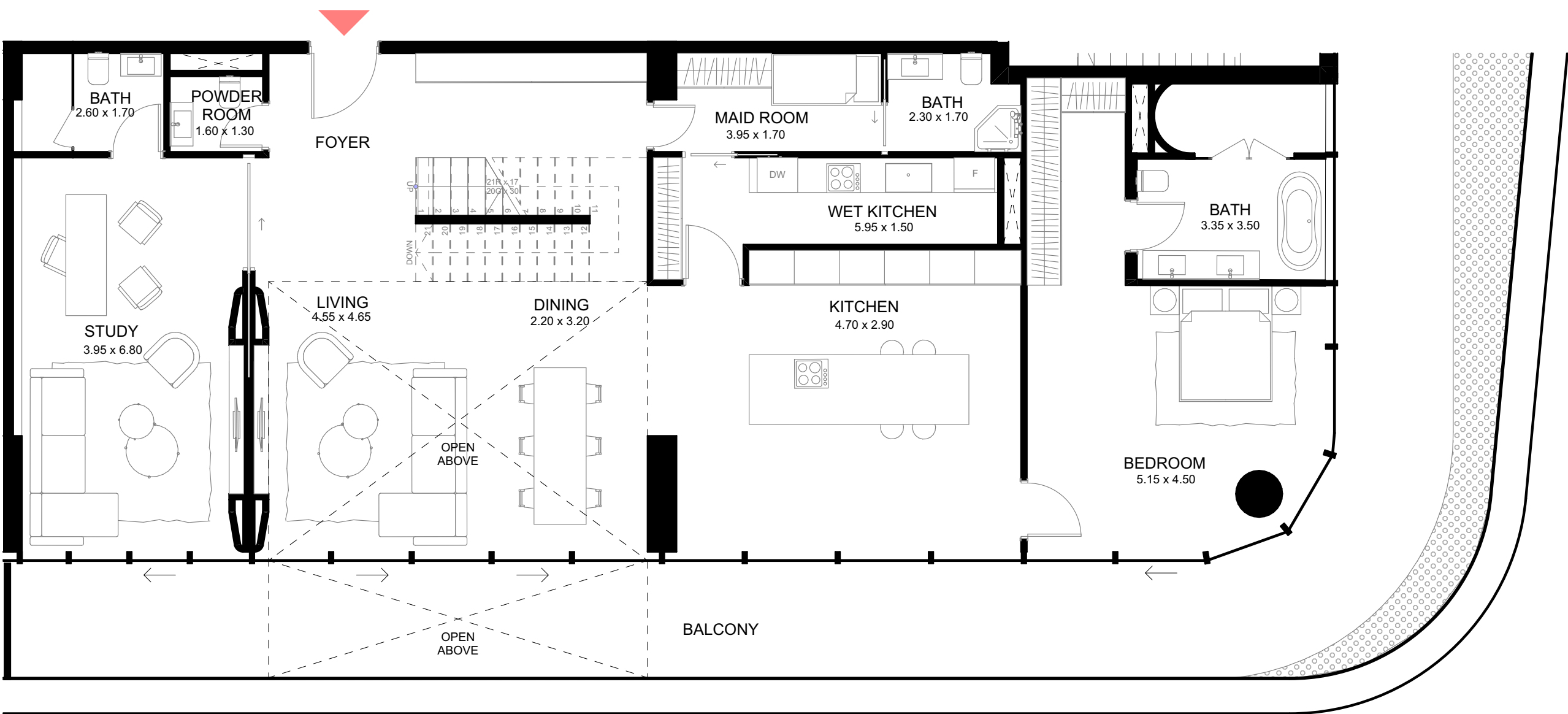
LOWER FLOOR PLAN
