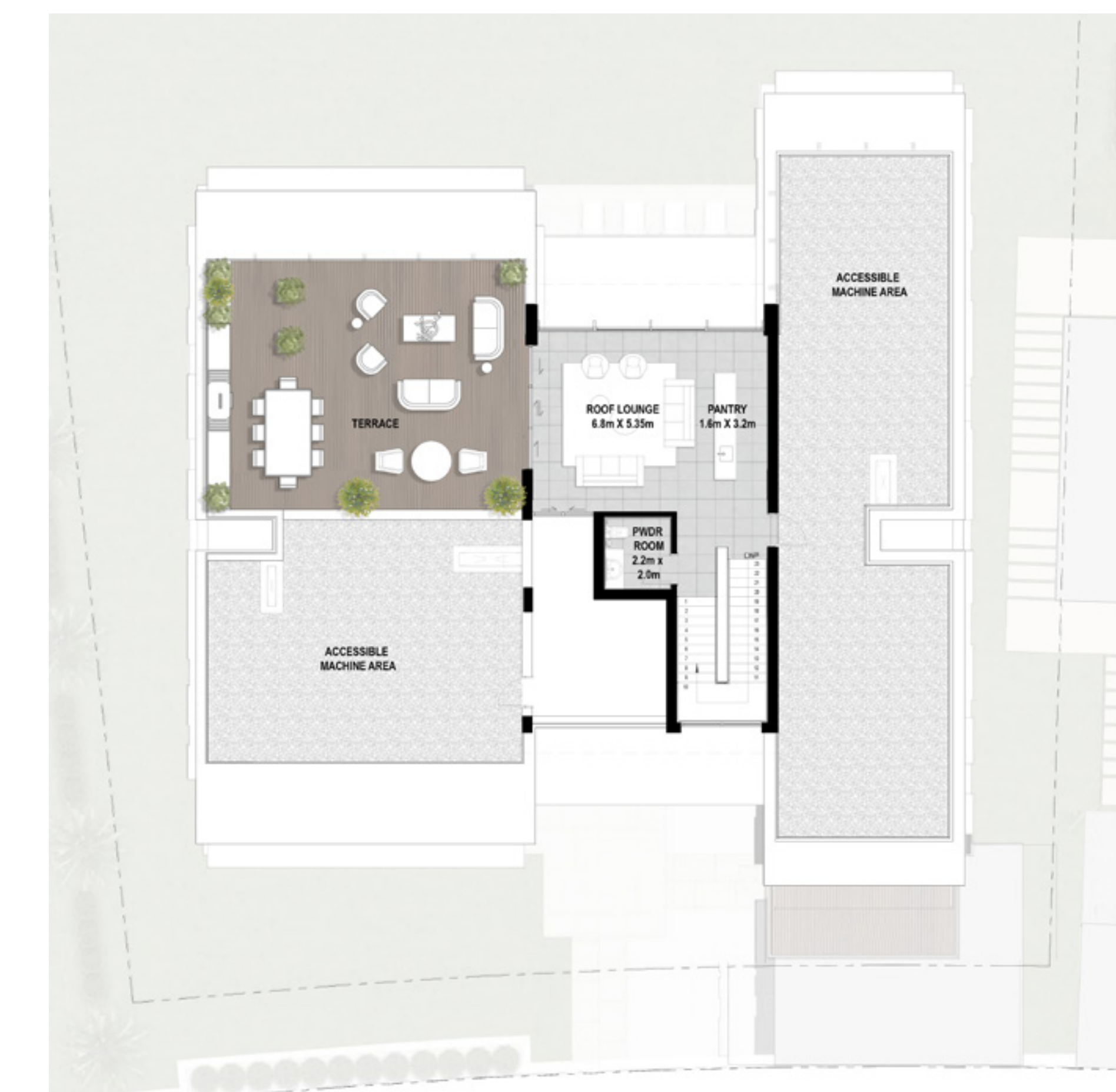
ROOF FLOOR
