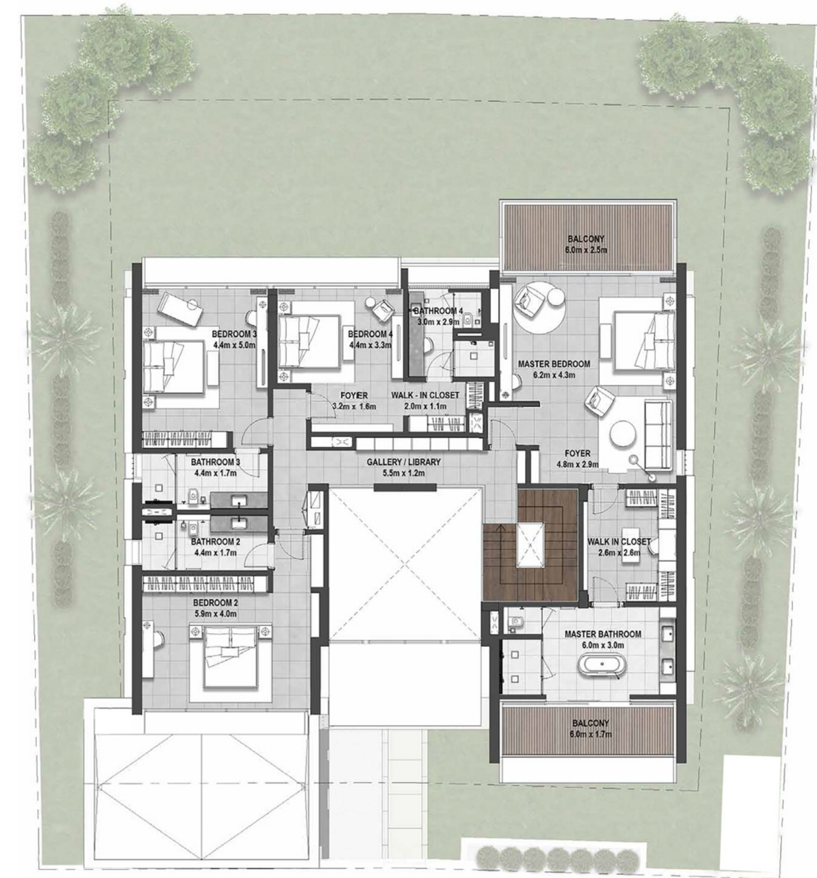
FIRST FLOOR
