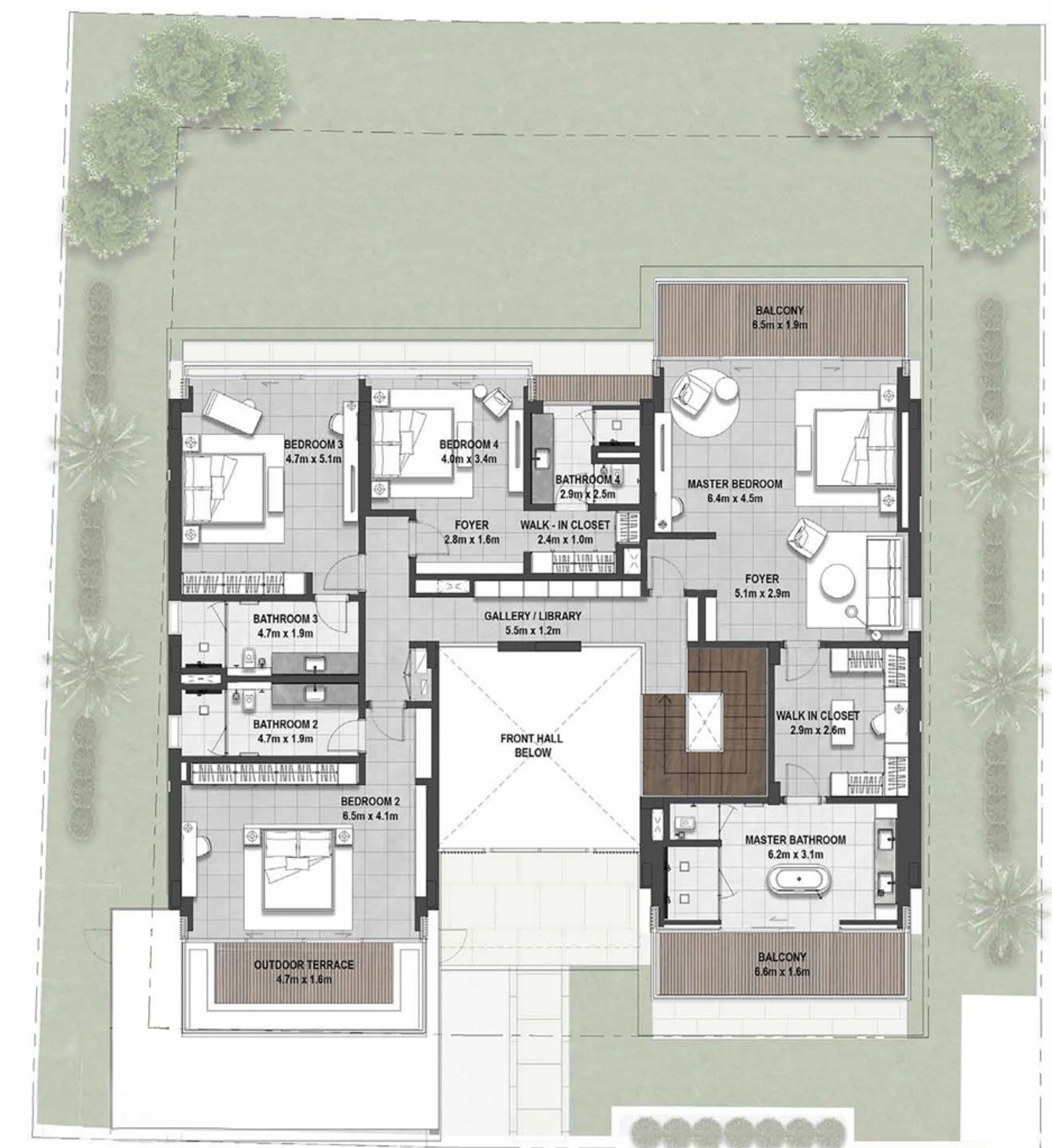
FIRST FLOOR
