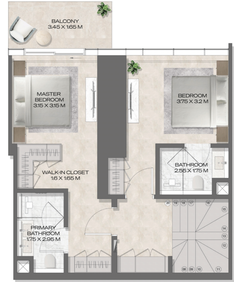
UPPER LEVEL
