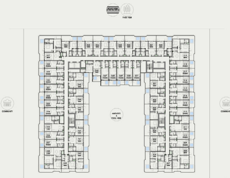
3rd Floor Plan Key Plan
