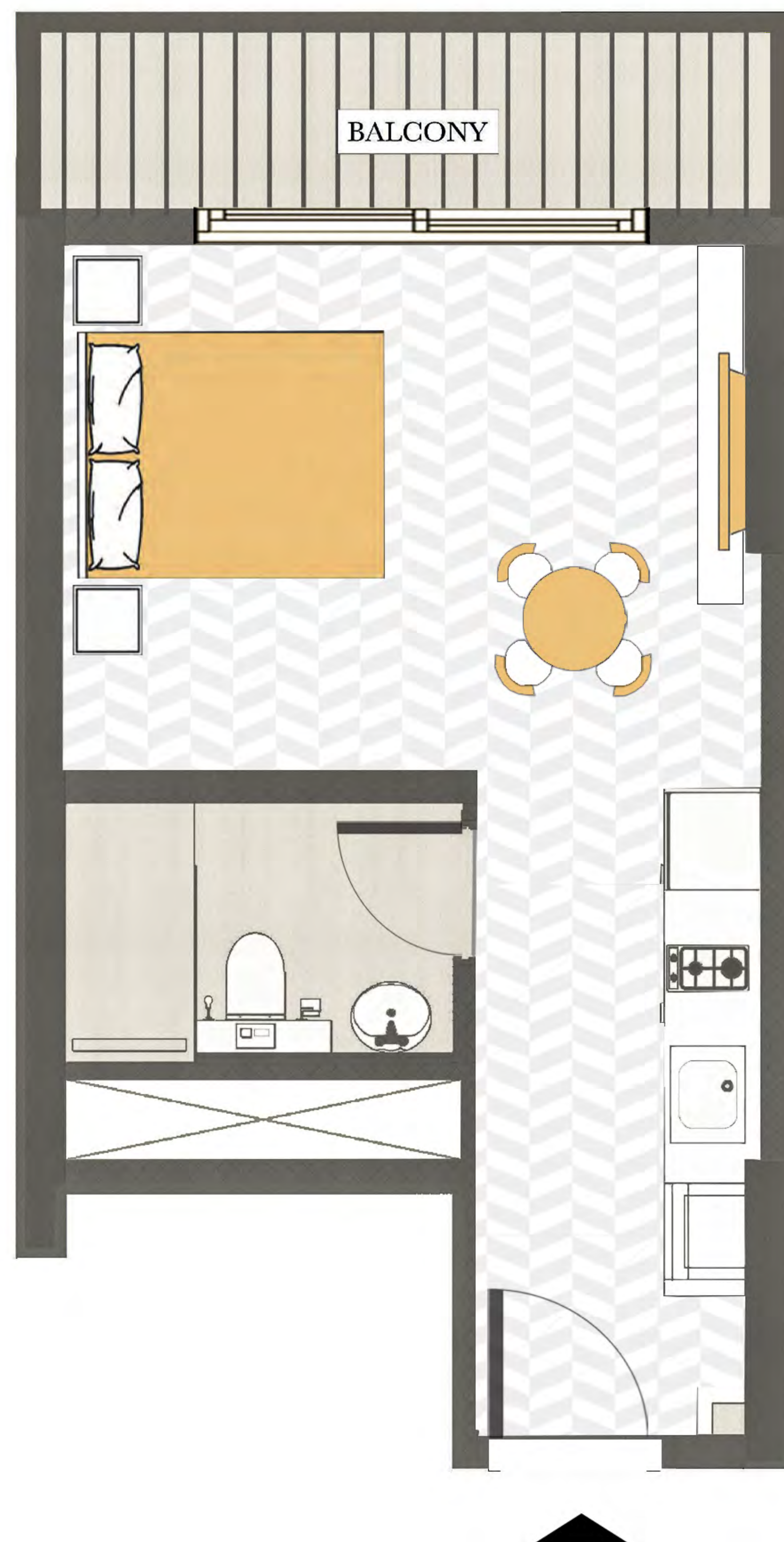
2 nd - 11 th Floor Plan
