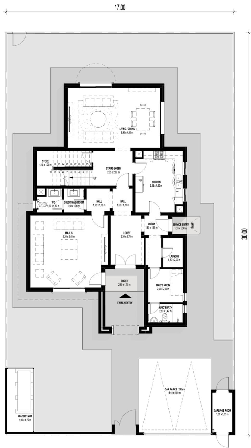
GROUND FLOOR
