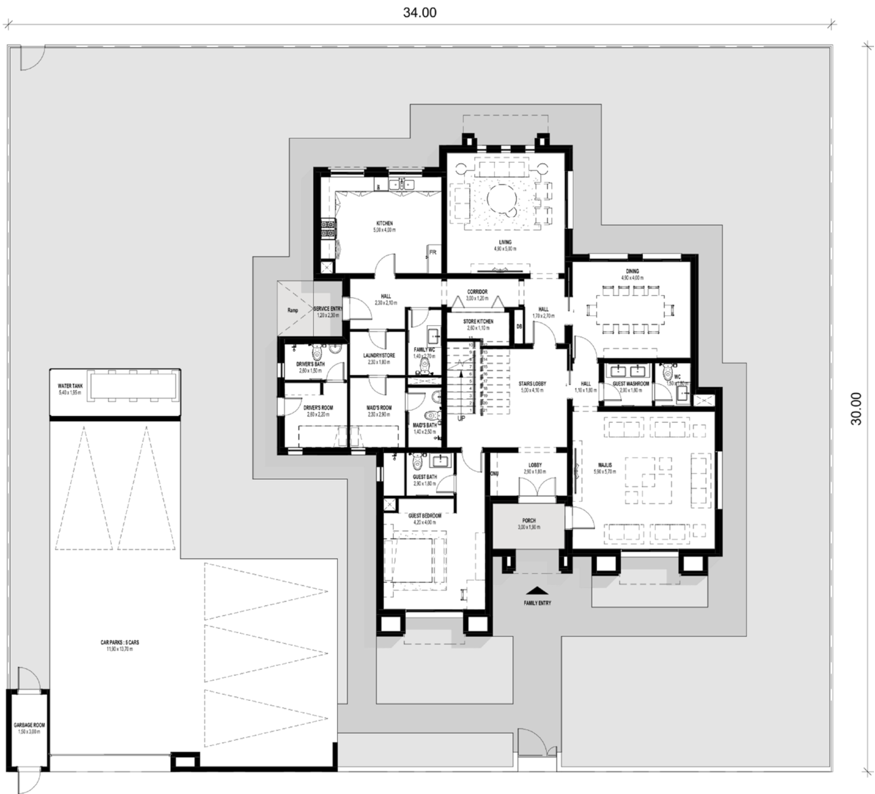
GROUND FLOOR
