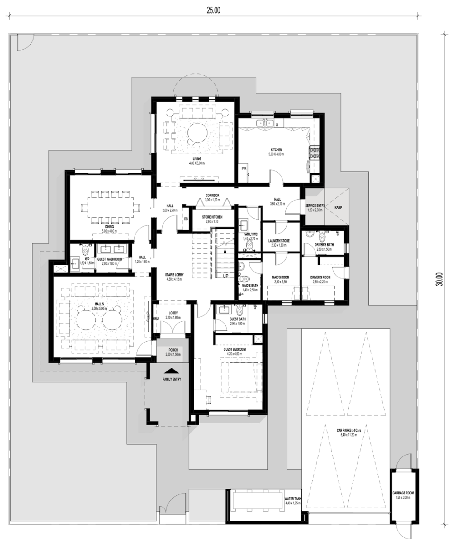
GROUND FLOOR
