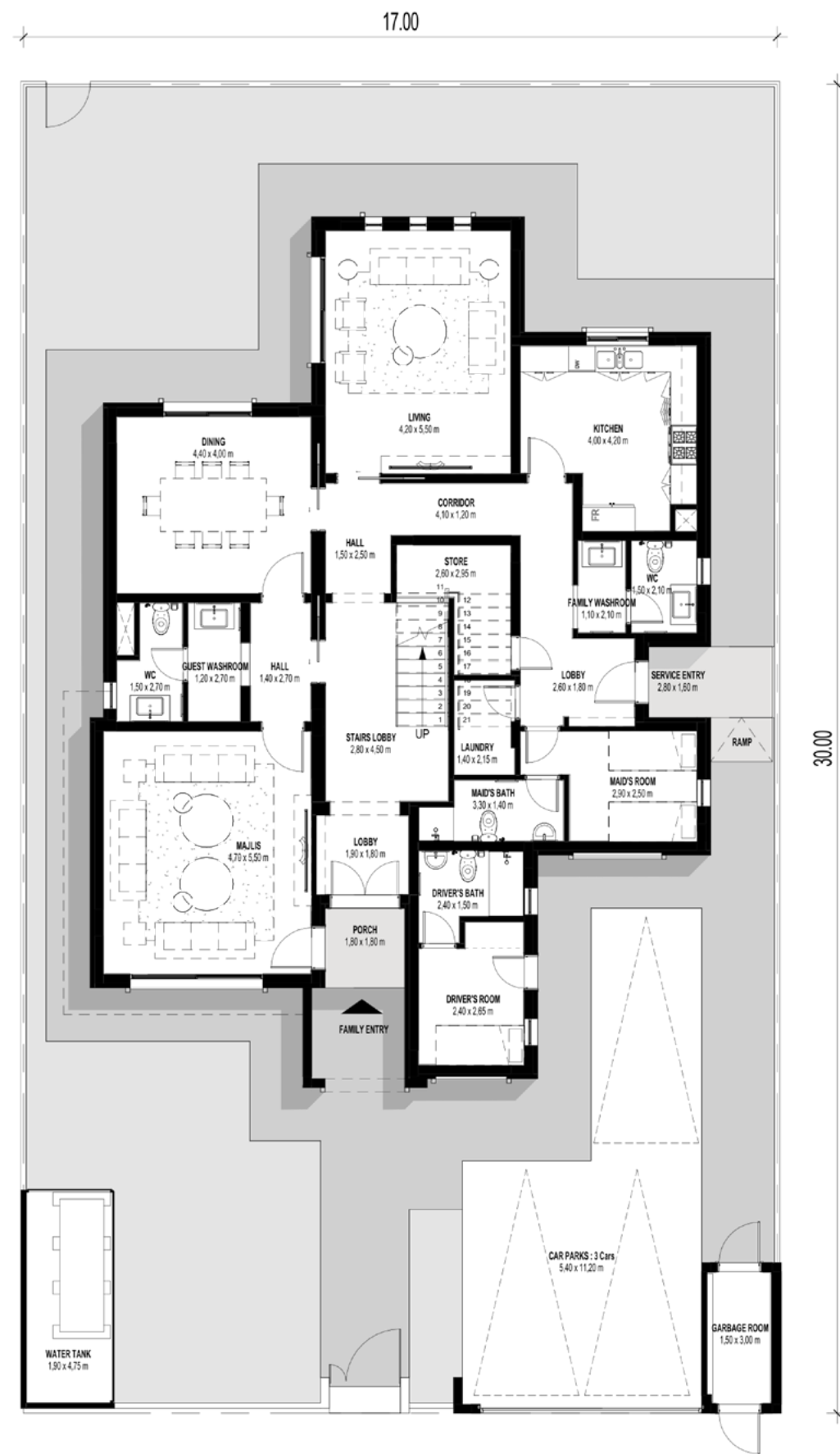
GROUND FLOOR
