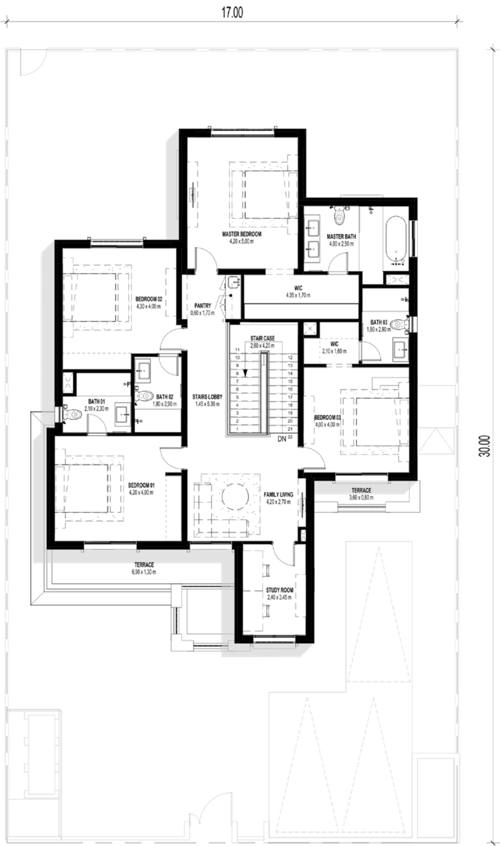
FIRST FLOOR
