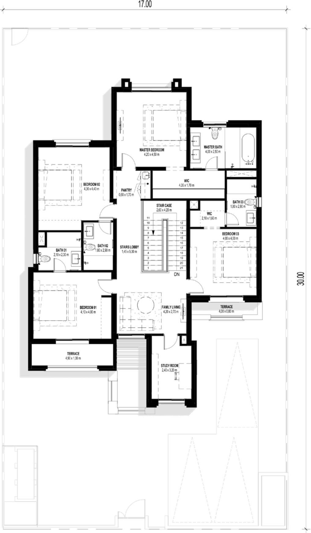
FIRST FLOOR
