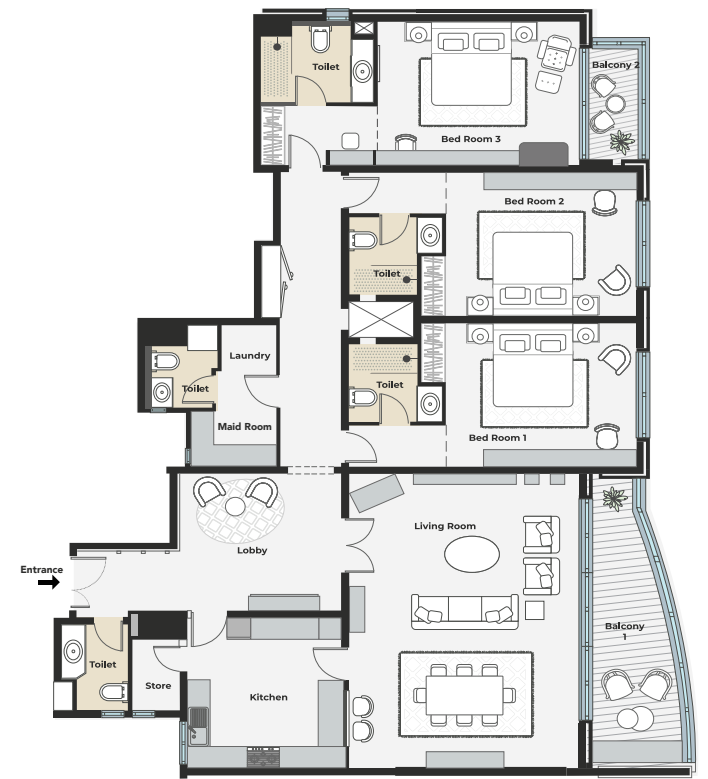
FLOOR PLAN
