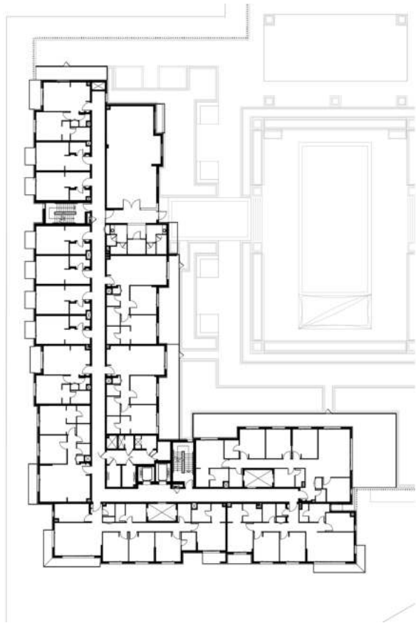
LEVEL 02
