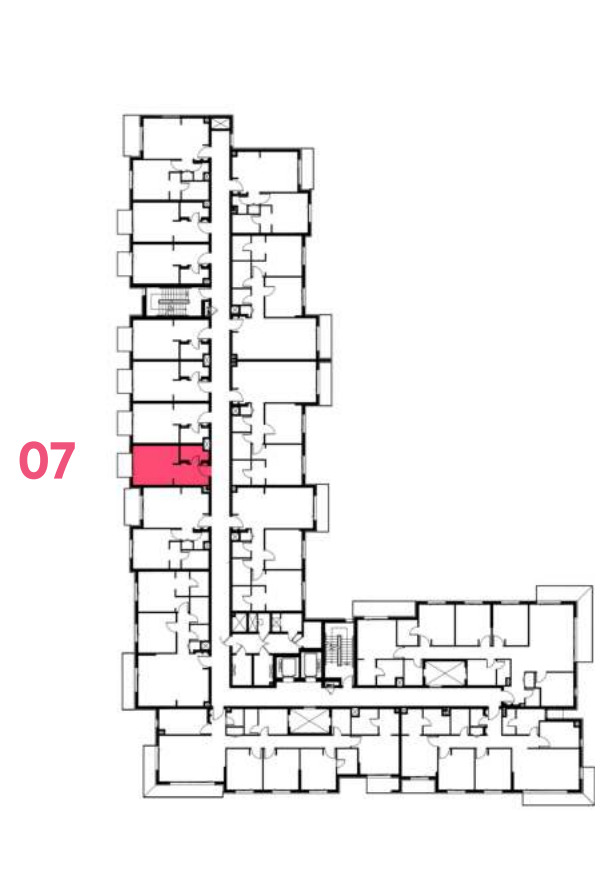
LEVEL 03,04,05
