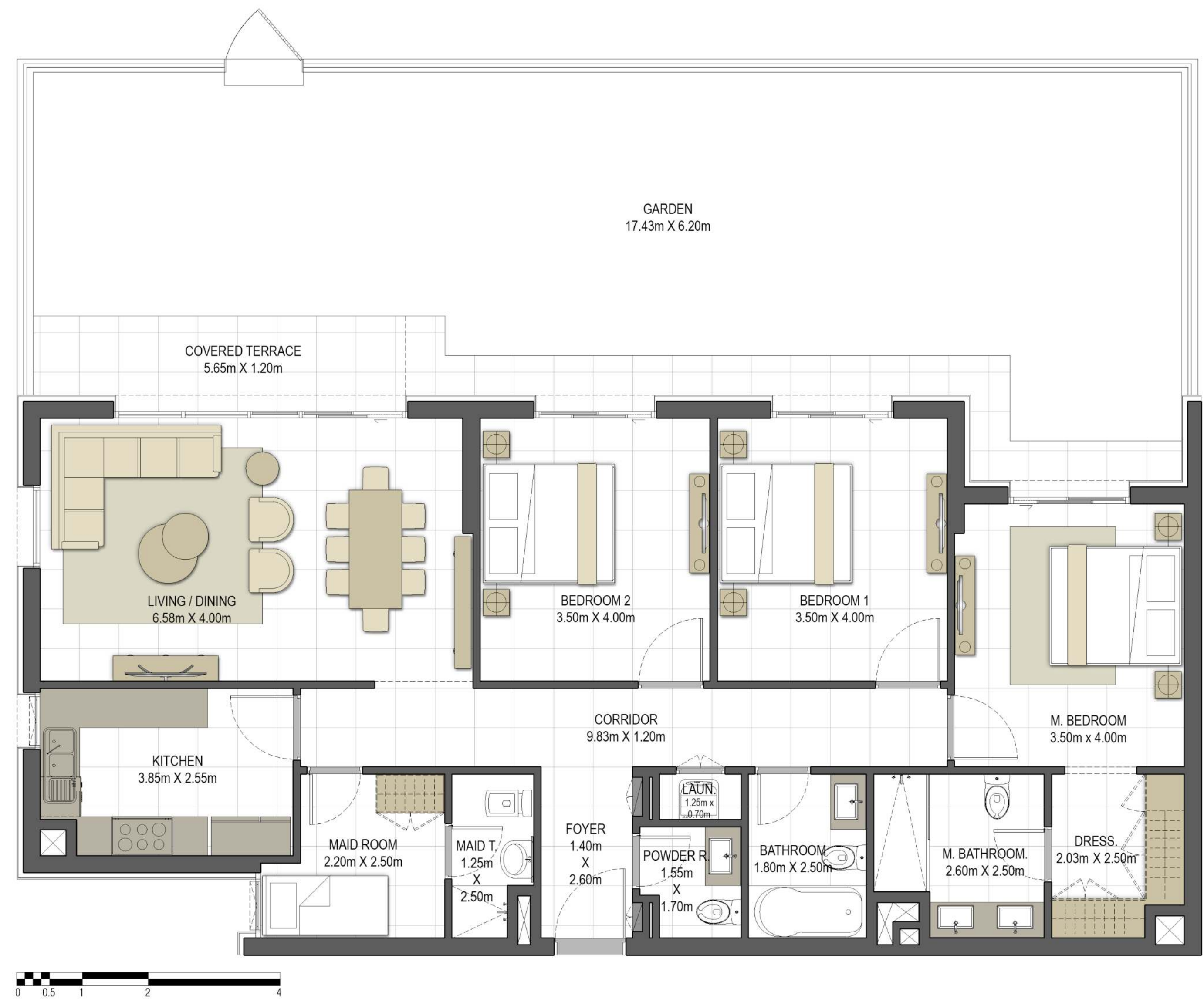
LEVEL 01
