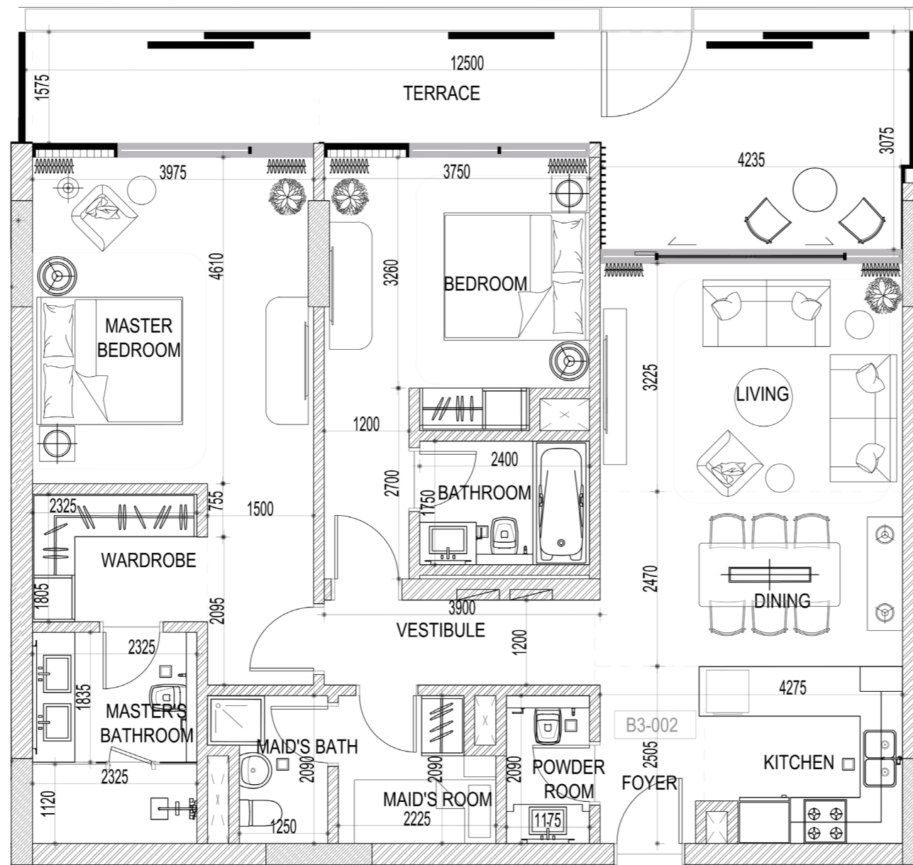
2 BED - APT 002
