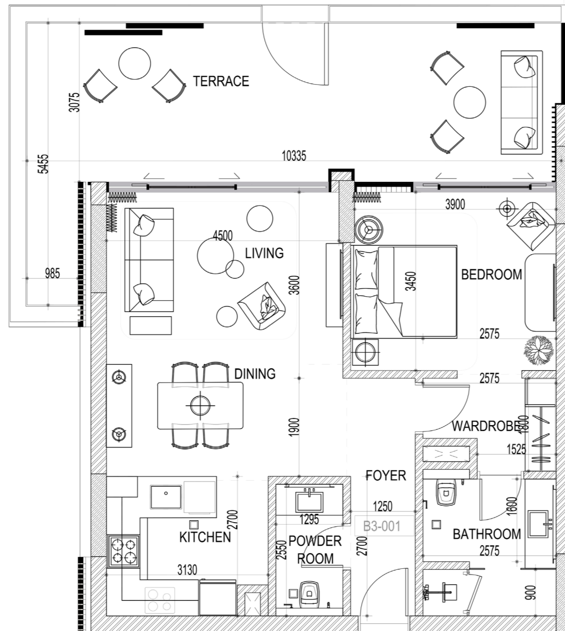
1 BED - APT 001
