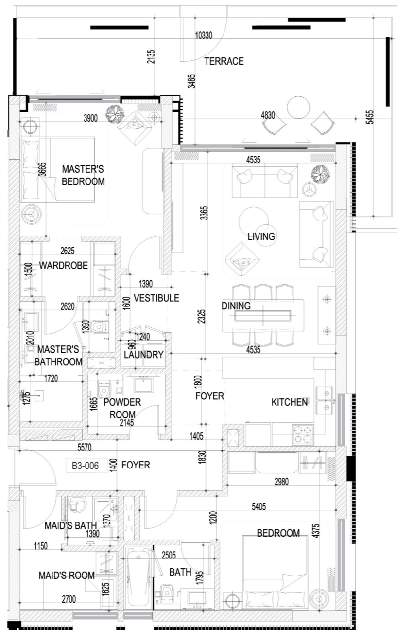
2 BED - APT 006
