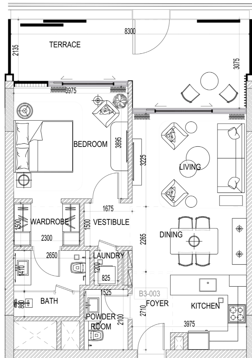
1 BED - APT 003
