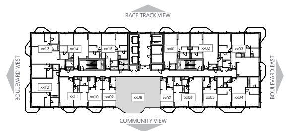
KEYPLAN - LEVEL 04 ( TYP. EVEN LEVELS UPTO L16)
