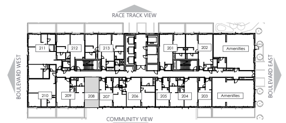
KEYPLAN - LEVEL 02
