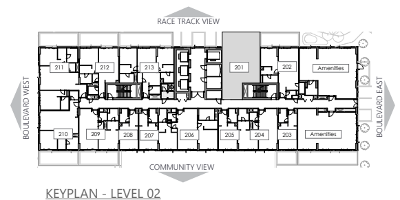
KEYPLAN - LEVEL 02
