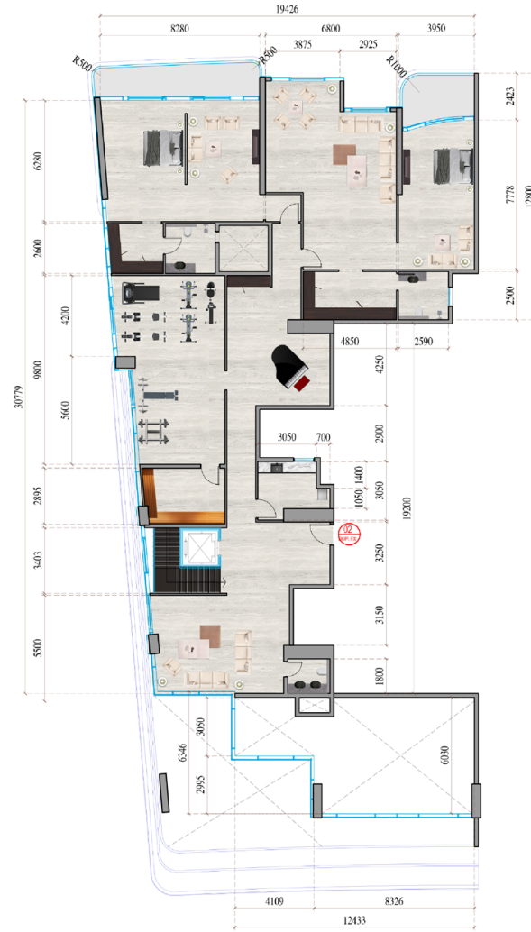
② 48th FLOOR PLAN DUPLEX 2 - UPPER FLOOR
