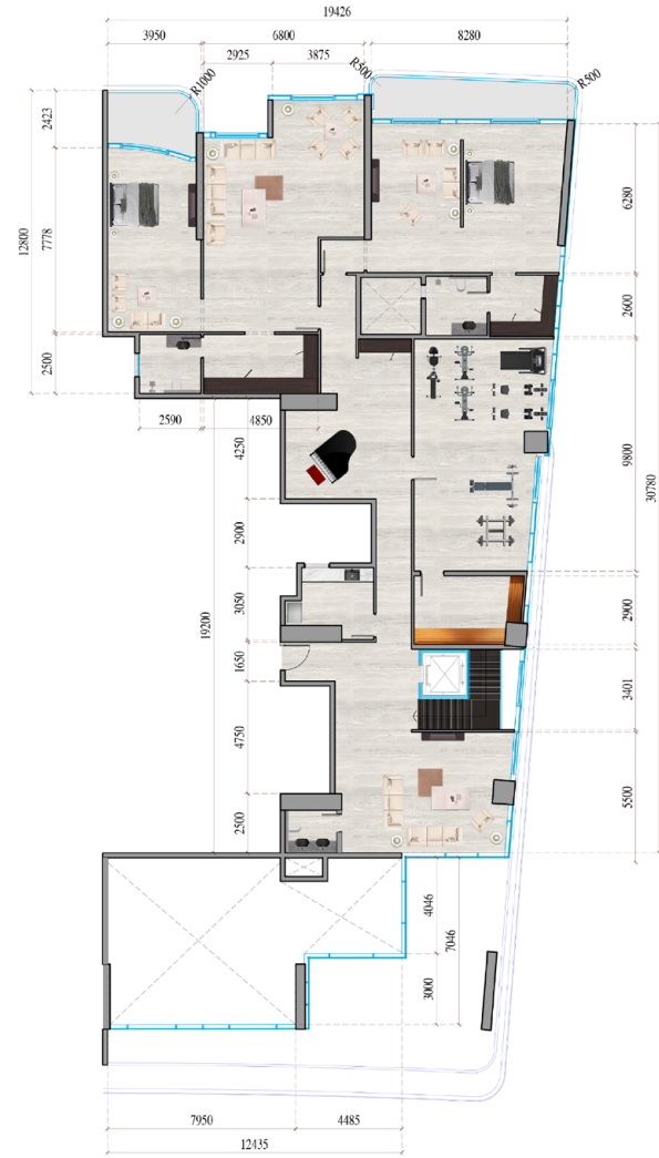
② 46th FLOOR PLAN DUPLEX 1 - UPPER FLOOR
