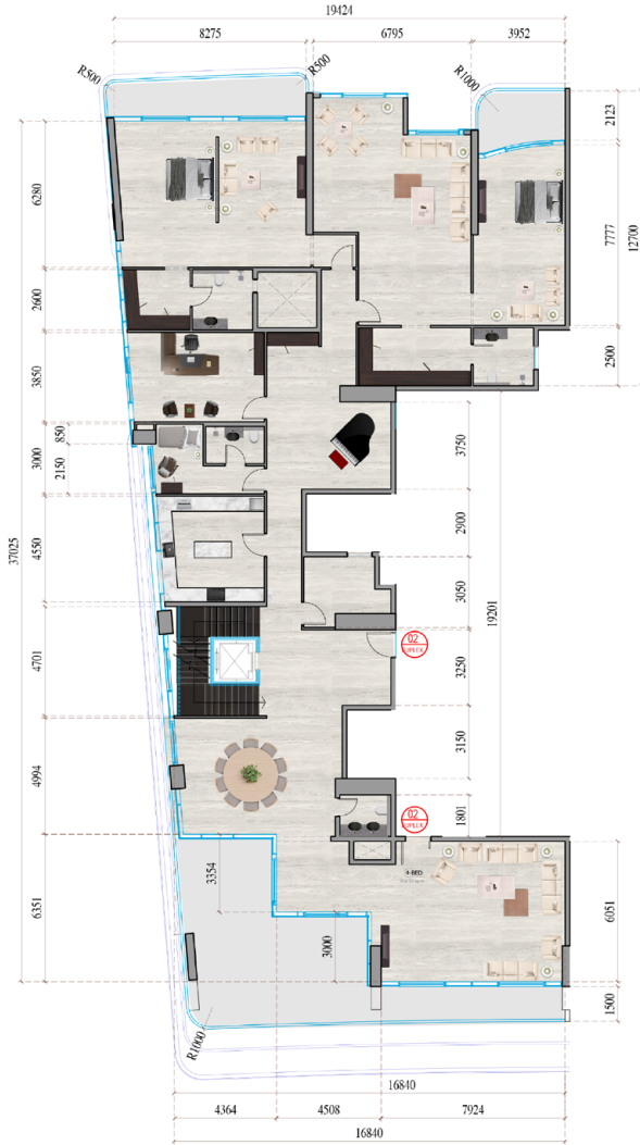
① 47th FLOOR PLAN DUPLEX 2 - LOWER FLOOR
