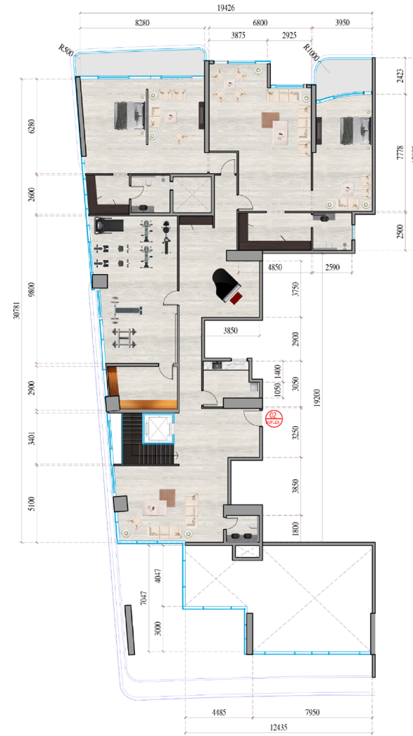
2 46th FLOOR PLAN DUPLEX 2 - UPPER FLOOR
