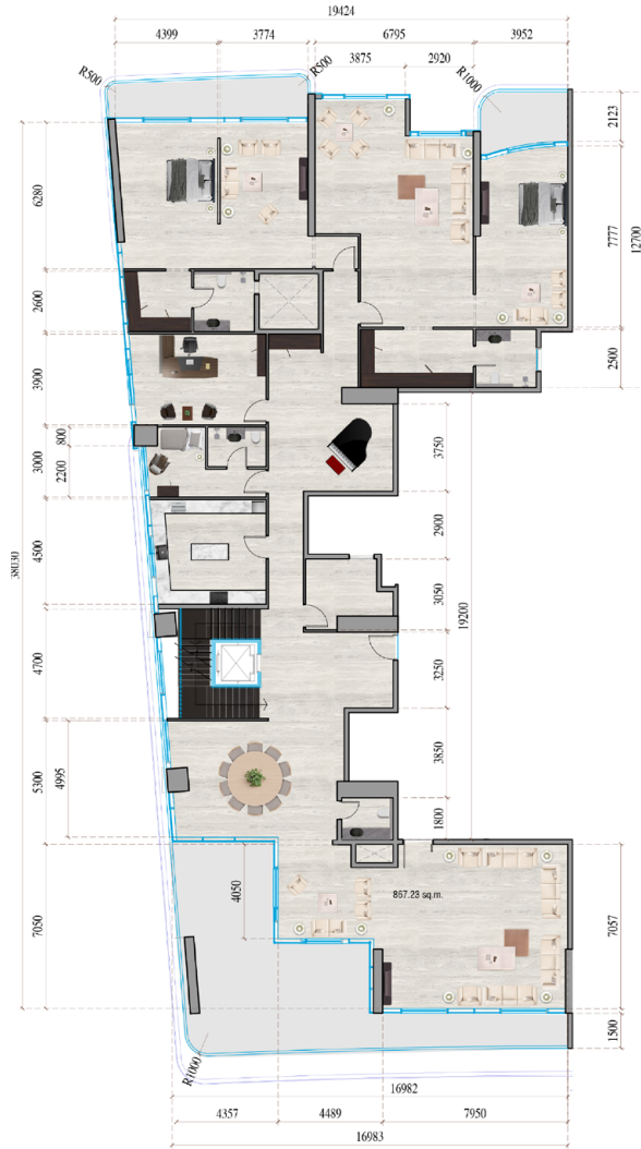
1 45th FLOOR PLAN DUPLEX 2 - LOWER FLOOR
