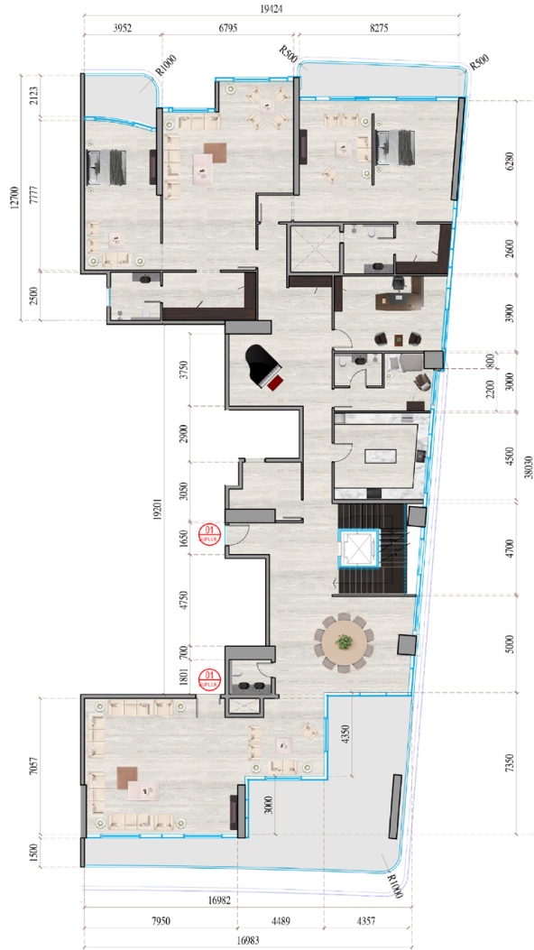
① 45th FLOOR PLAN DUPLEX 1 - LOWER FLOOR
