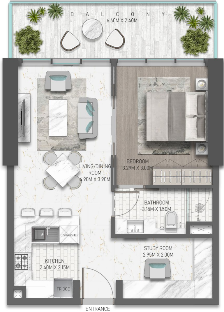
1 BEDROOM TYPE A-2 SALEABLE AREA: 725 SQFT
