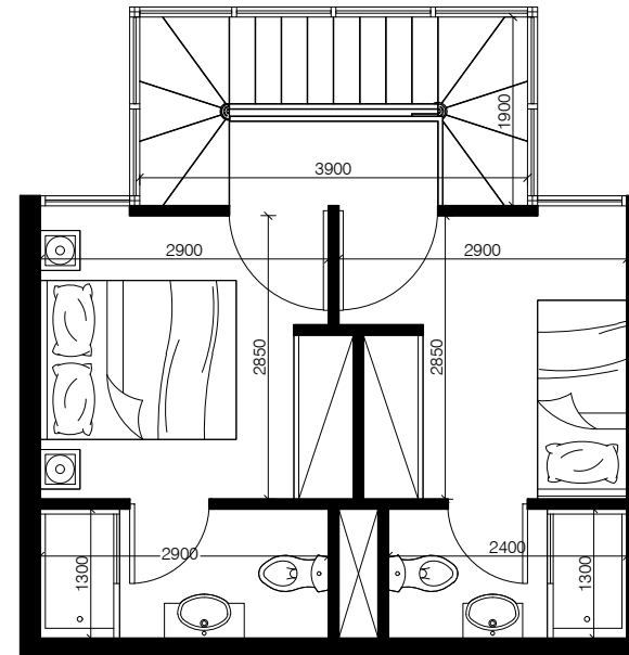
Upper level
