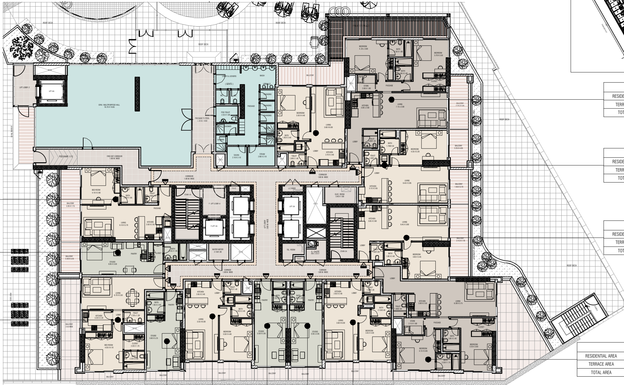
KEY PLAN
