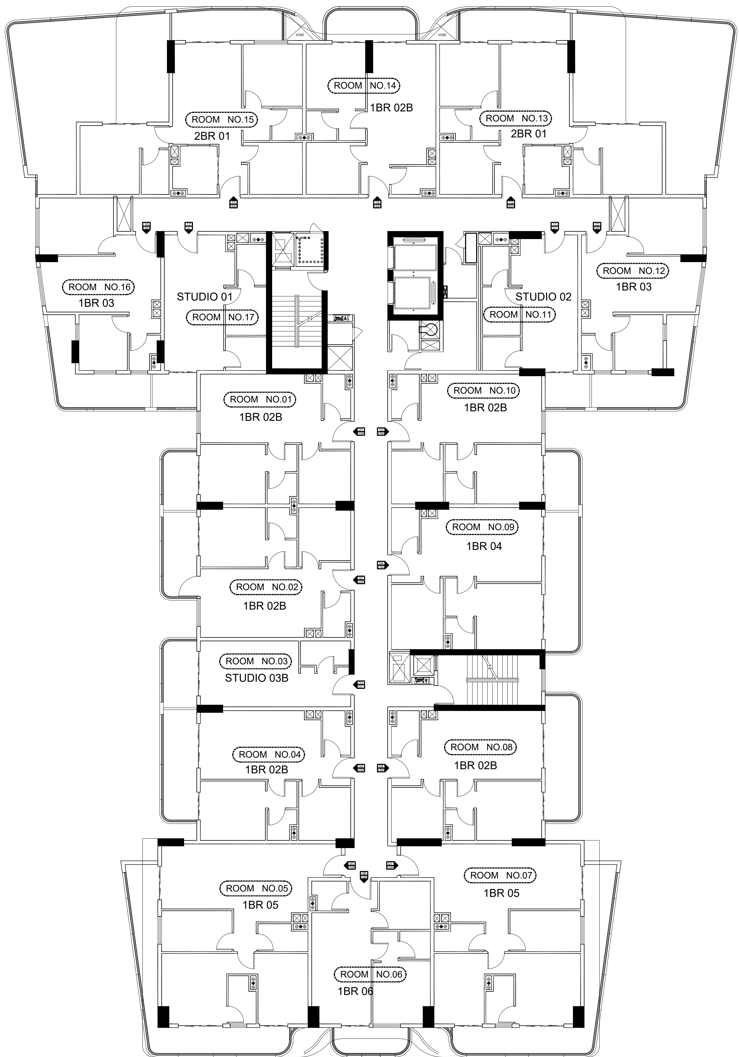
10th FLOOR PLAN
