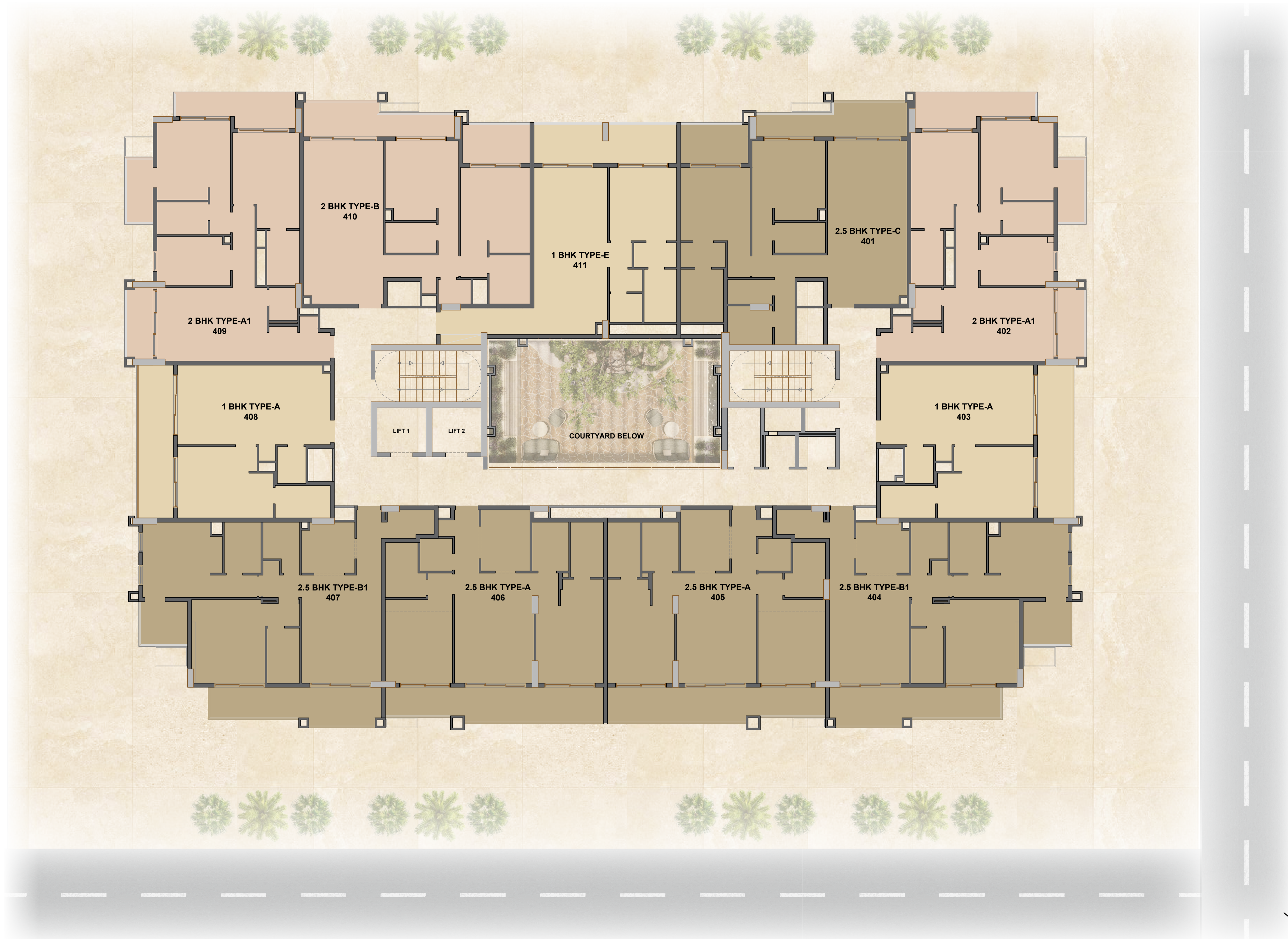
Fourth floor plan
