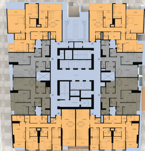
11th, 21st, 31st, 41th FLOOR PLAN SCALE: 1:100
