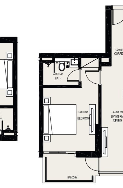
ONE BEDROOM 16
