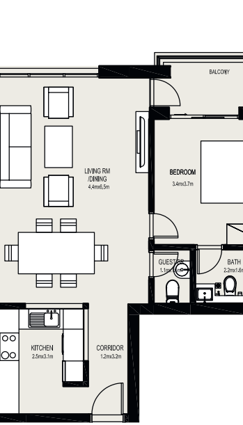
ONE BEDROOM 09
