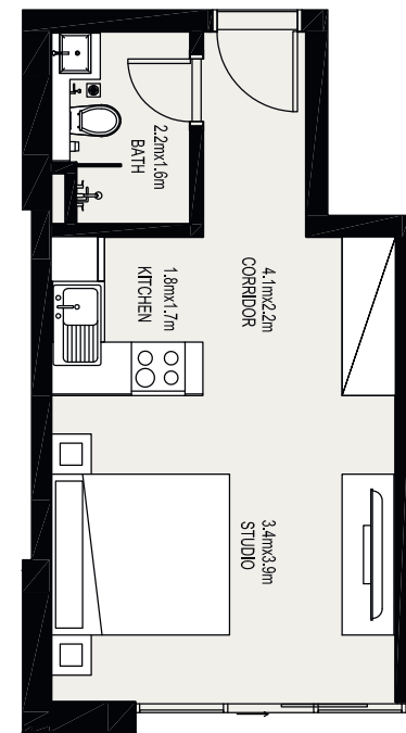
STUDIO 04/05
