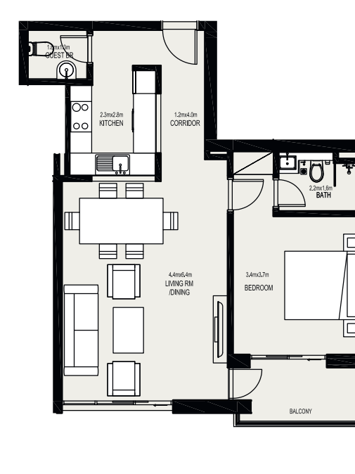
ONE BEDROOM 17
