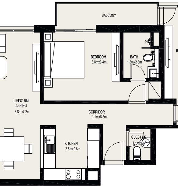
TWO BEDROOM 13/14
