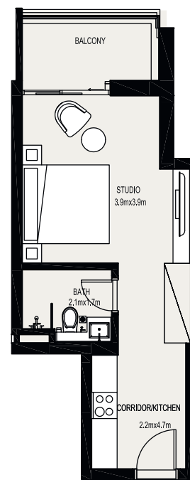
STUDIO 11
