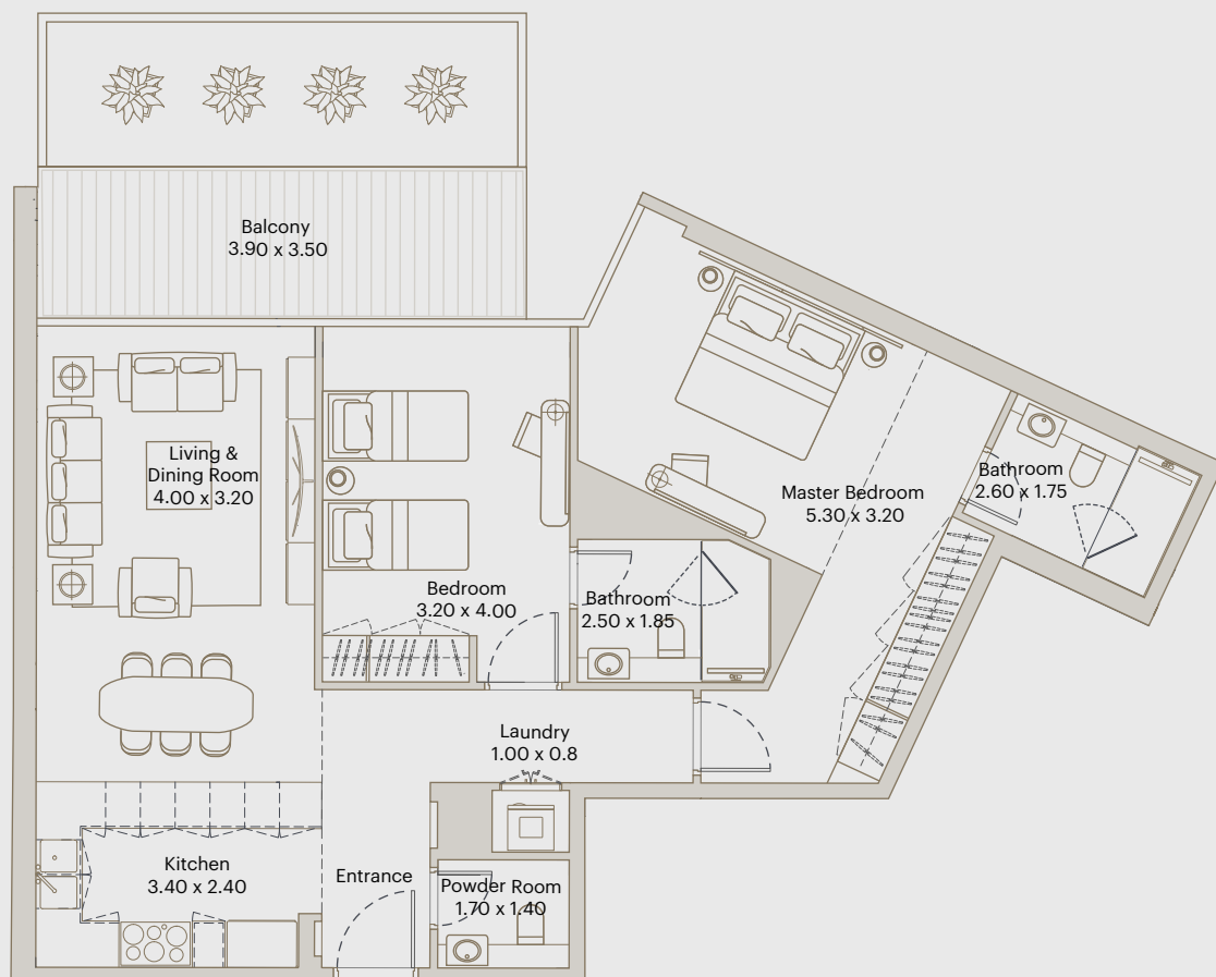
FLAT 17 @ 3RD, 5TH, 7TH, 9TH, 11TH, 13TH, 15TH & 17TH FLOOR
