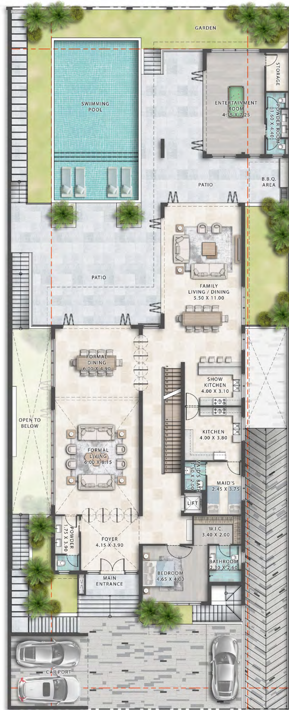
GROUND FLOOR
