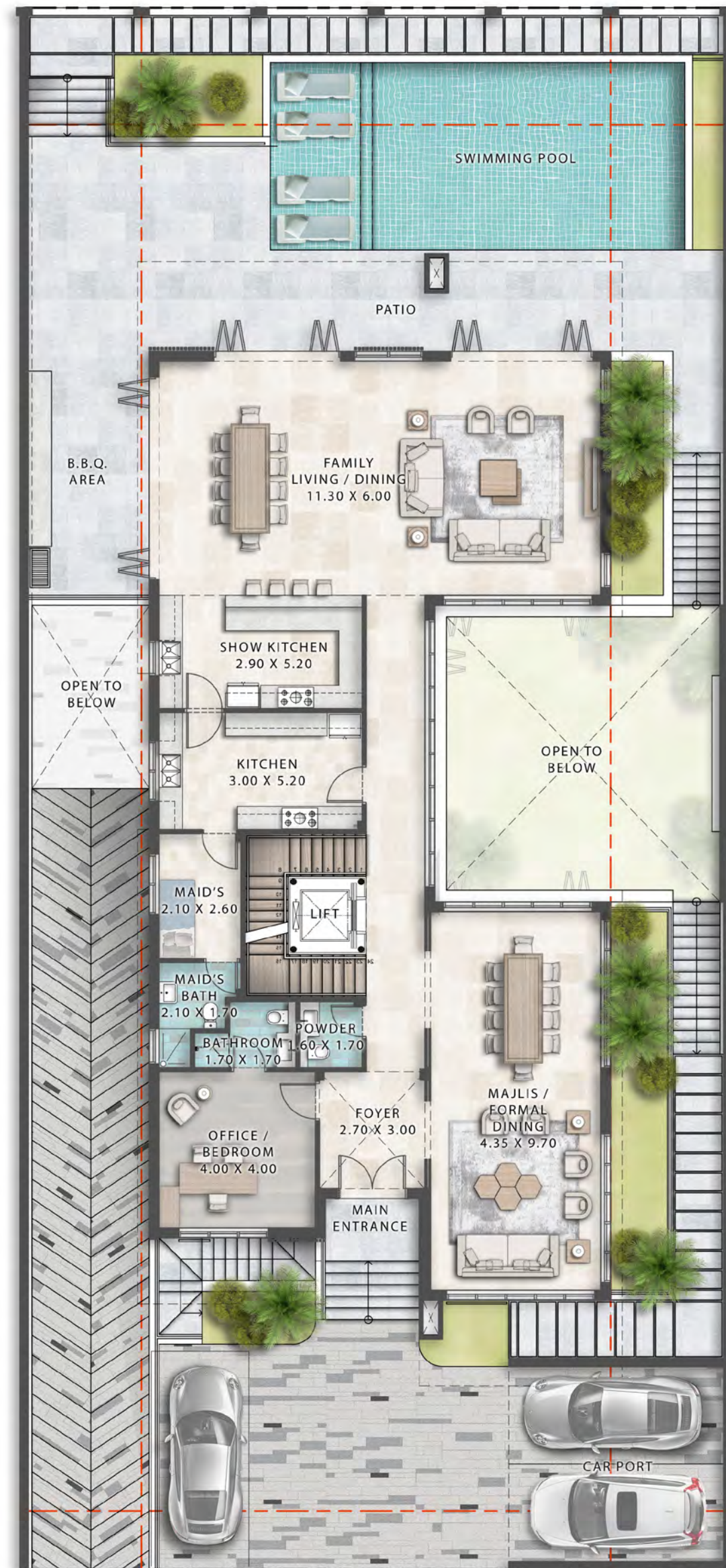
GROUND FLOOR
