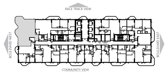
KEYPLAN - LEVEL 03 (TYP. ODD LEVELS UPTO L17)
