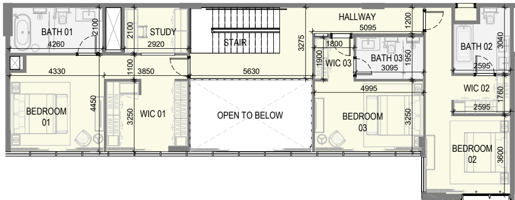
LEVEL 30
