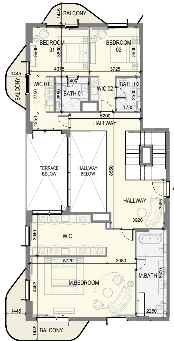
LEVEL 30
