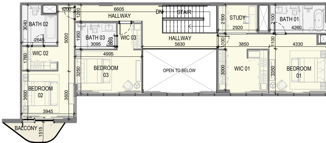
LEVEL 30
