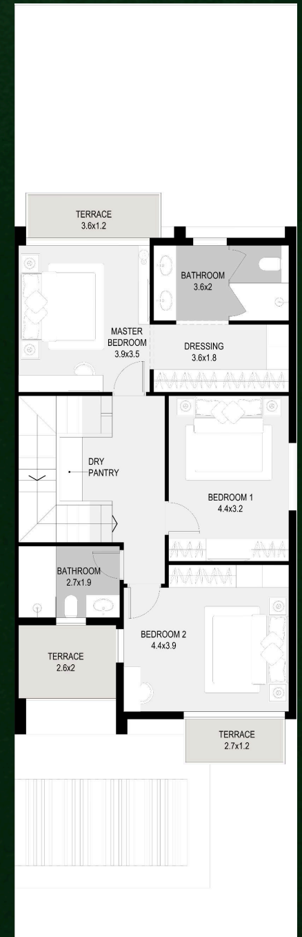
FIRST FLOOR
