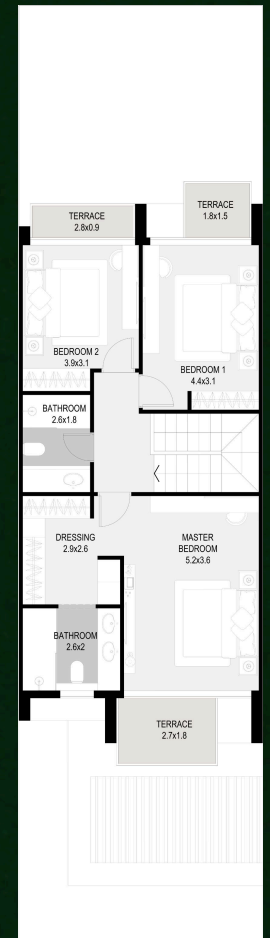
FIRST FLOOR
