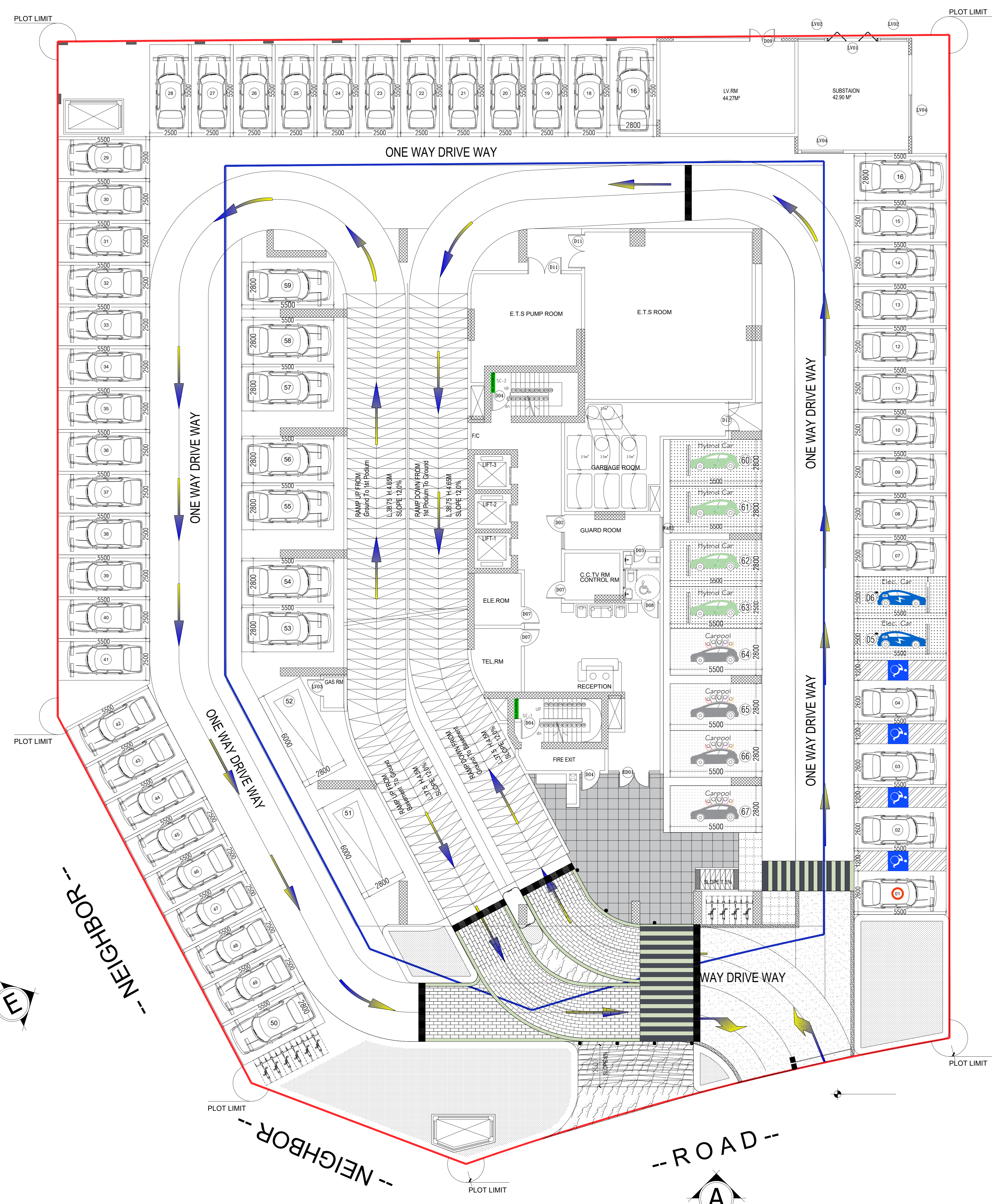
Ground FLOOR PLAN Total parking 67.nos
